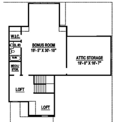
SECOND FLOOR 939 SQ. FT.
