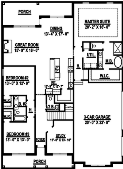
FIRST FLOOR 2,298 SQ. FT
