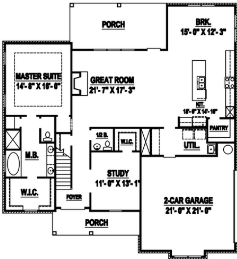
FIRST FLOOR 1,802 SQ. FT
