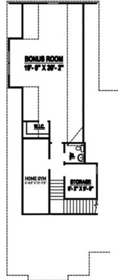
SECOND FLOOR 769 SQ. FT
